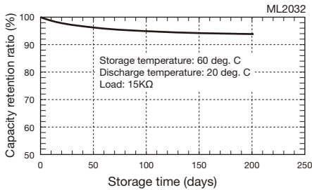
Fig. 3 Low Self-discharge
